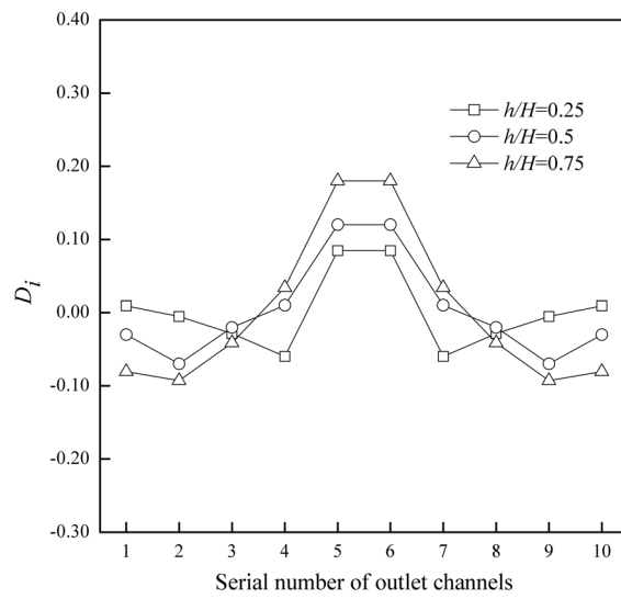
5 Fig. 14. Relative flowrate deviation for optimized configurations with different baffle locations. N=10 ;
