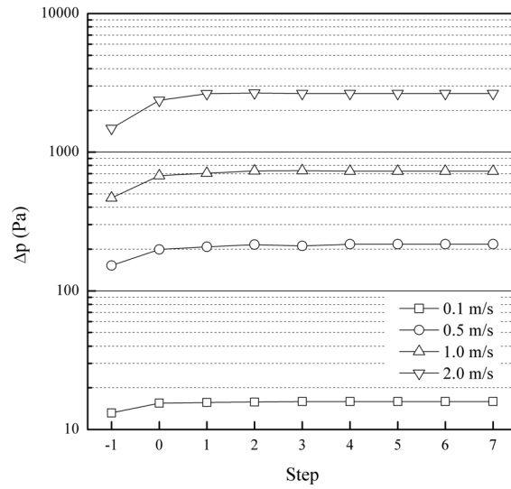
2 Fig. 13. Influence of inlet flowrate on the pressure drop in the baffled fluid distributor. N=10 ; M=10 ;
