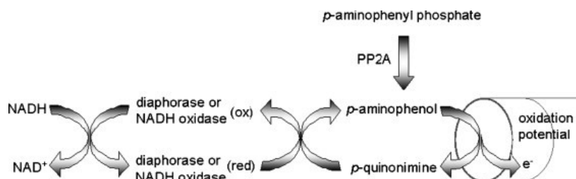
Figure 2. Scheme of the enzymatic signal amplification for the detection of the PP2A activity (Campas et al., 2008). The detection principle is based on the dephosphorylation of non-electroactive p-APP by PP2A, the oxidation of the corresponding electroactive p-aminophenol to p-iminoquinone (p-IQ) on the electrode surface and the regeneration of p-IQ by diaphorase, which requires NADH as substrate
