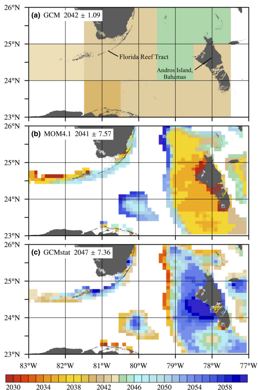
Fig. 5 Projected timing in years of the onset of annual severe bleaching ( >8 DHW) for the Florida Reef Tract and the Bahamas for: (a) the ensemble of Global Climate Models (GCMs, see Table S1 for list) at GCM-resolution ( \sim 1^\circ ), (b) dynamical downscaling through using GCM outputs to force the GFDL Modular Ocean Model (MOM4.1, \sim 0.1^\circ or \sim 11 km resolution), and (c) statistically downscaling GCM outputs by replacing the model mean and annual cycle for SST with observed data from 1982 to 2008. For each plot, mean year is shown \pm 1 standard deviation.
