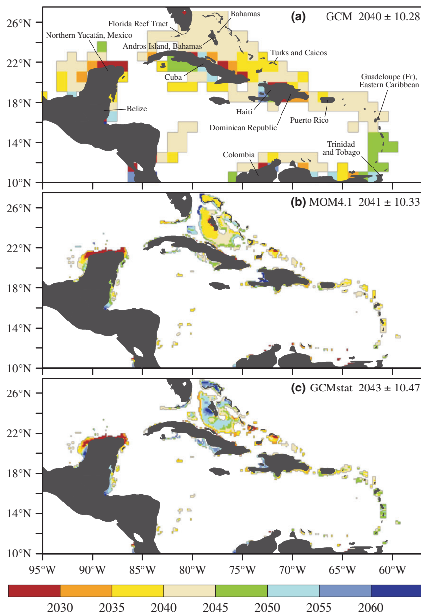
Fig. 1 Projected timing in the onset of annual severe bleaching (>8 DHW) in years for: (a) the ensemble of Global Climate Models (GCMs, see Table S1 for list) at model resolution (1° × 1°), (b) dynamical downscaling through using GCM outputs to force the GFDL Modular Ocean Model (MOM4.1, ~0.1° resolution), and (c) statistically downscaling GCM outputs by replacing the model mean and annual cycle for SST with observed data from 1982 to 2008 re-gridded to the scale of MOM4.1. For each plot, mean year is shown ±1 standard deviation.
