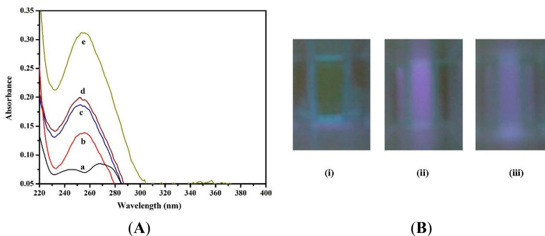
Figure 2. (A) UV absorption spectra of (a) TiO 2 ; (b) Aptamer; (c) Aptamer-target complex (in absence of TiO 2 ); (d) Aptamer-target complex (in presence of TiO 2 ); and (e) Aptamer-TiO 2 complex; (B) Fluorescence imaging of (i) FAM-aptamer; (ii) aptamer-TiO 2 ; and (iii) aptamer-target complex (in presence of TiO 2 ).
