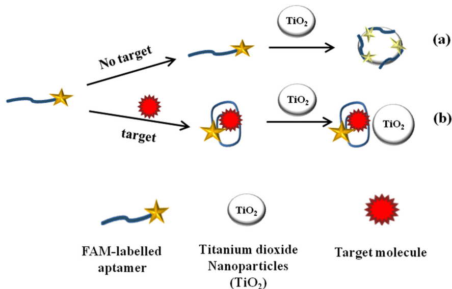
Figure 1. Schematic representation of TiO 2 quenching based sensing platform for target molecule detection. (a) In the absence of target analyte, adsorption of FAM-labeled aptamer on TiO 2 surface led fluorescence quenching; (b) In the presence of target analyte, the anti-parallel G-quadruplex structure form decrease adsorption and fluorescence recovered.
