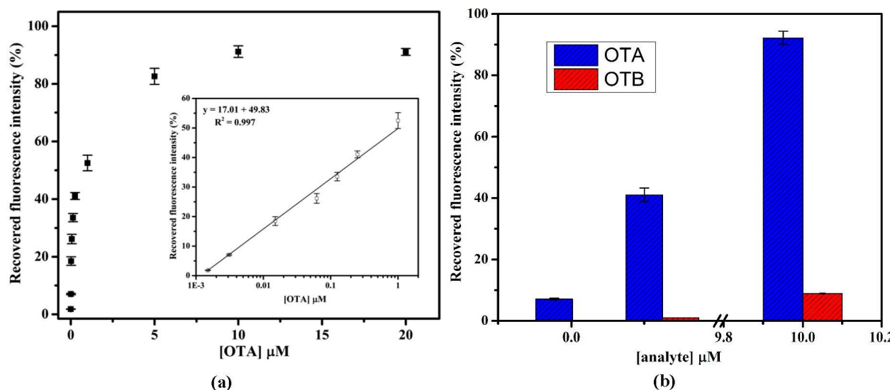
Figure 5. (a) Calibration graph for OTA analysis in HBB, pH 7.4 showing recovered fluorescence intensity percentage against OTA concentration. Inset showing the linear fit graph; (b) Bar graph representation of specificity studies of aptamer with OTB. Error bars were obtained from three parallel experiments.
