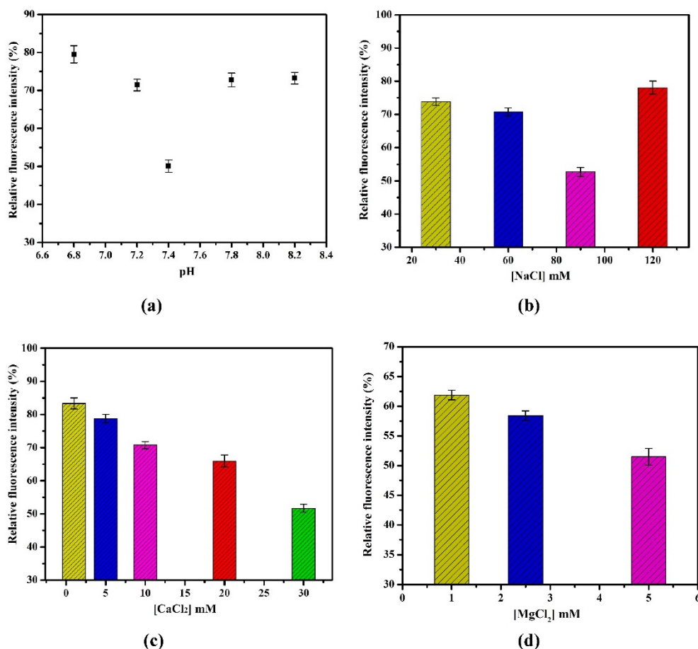
Figure 4. (a) Effect of pH (6.8–8.2) in HBB on quenching performance of TiO 2 ; (b) Effect of NaCl concentrations (30, 60, 90 and 120 mM) on quenching performance of TiO 2 ; (c) Effect of CaCl 2 concentrations (1, 5, 10, 20 and 30 mM) on quenching performance of TiO 2 ; (d) Effect of MgCl 2 concentrations (1, 2.5 and 5 mM) on quenching performance of TiO 2 . The error bars were obtained from three parallel measurements.
