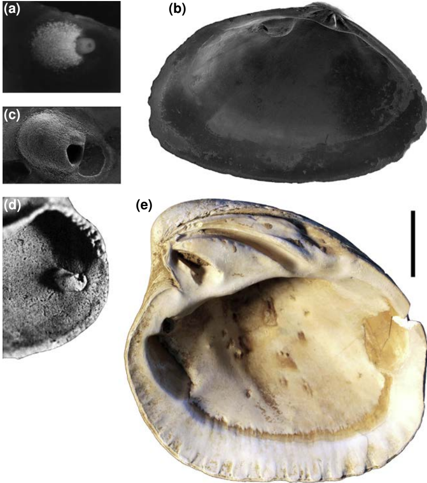
Figure 2 Shell structures (igloo-shaped concretions, shell pits) which have been linked with gymnophallid trematodes (Digenea) in extant and fossil bivalves. (a) Metacercaria lodged in live position into an igloo-shaped calcareous covering of Gaimardia trapesina (MLP 5659) from Beagle Channel in Ushuaia; note the noncalcified area around the anterior end of the larva (photo: Cristian Ituarte; refigured from Ituarte et al. (2005).); (b) Scanning electron micrograph of a left valve of Cyamiomactra sp. from a Holocene sample of Río Varela (Tierra del Fuego) showing a single igloo-shaped covering just below the anterodorsal margin (Photo: Cristián Ituarte; refigured from Ituarte et al. (2005).); (c) Upper view of an igloo-shaped covering in G. trapesina (MLP 5659) from Beagle Channel in Ushuaia showing the non-calcified area in front of the igloo opening (Photo: Cristian Ituarte; refigured from Ituarte et al. (2005).); (d) Igloo-shaped concretion found close to posterior adductor muscle scar in the Silurian bivalve Nuculodonta gotlandica (SGU Type 1030) from the Halla Formation of Gotland (Modified from Liljedahl (1994).); (e) Interior of right valve of Venericor clarendonensis (NHMUK PI TB 14236) from the Eocene (subdivision B2 of the London Clay) with irregular shell deformations and shell pits interpreted to have been produced in response to digenean trematode infestation. Photo courtesy of Jon Todd; compare Todd and Harper (2011).
