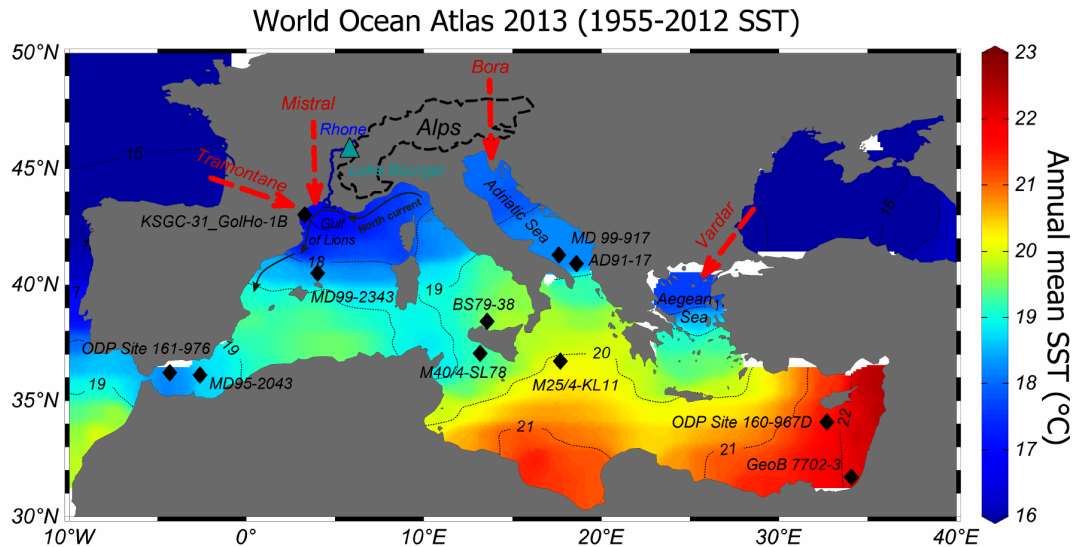
Figure 1. Map of the Mediterranean annual mean SSTs ( ^{\circ}\text{C} ; 1955 and 2012) from World Ocean Atlas 2013 ( http://odv.awi.de/de/data/ocean/world_ocean_atlas_2013/ ) plotted using Ocean Data View (Brown, 1998). The location of the KSGC-31_GolHo-1B core and other sites discussed in the text are also reported (from West to East): ODP Site 161–976, Alboran Sea (Martrat et al., 2014); MD95-2043, Alboran Sea (Cacho et al., 2001); MD 99-2343, Balearic basin (Frigola et al., 2007); M40/4-SL78, Ionian Sea (Emeis et al., 2003); BS79-38, Southern Tyrrhenian Sea (Cacho et al., 2001); MD90-917, Southern Adriatic Sea (Essallami et al., 2007); M25/4-KL11, the Ionian Sea (Emeis et al., 2003); AD91-17, Southern Adriatic Sea (Giunta et al., 2001); ODP Site 160-967D, Levantine basin (Emeis et al., 2000); GeoB 7702-3, Levantine basin (Castañeda et al., 2010). The location of Lake Bourget in France (LDB01-1 and LDB04-1 cores) is also shown (Arnaud et al., 2012). The main winds blowing in the Mediterranean Sea are shown by red arrows.
