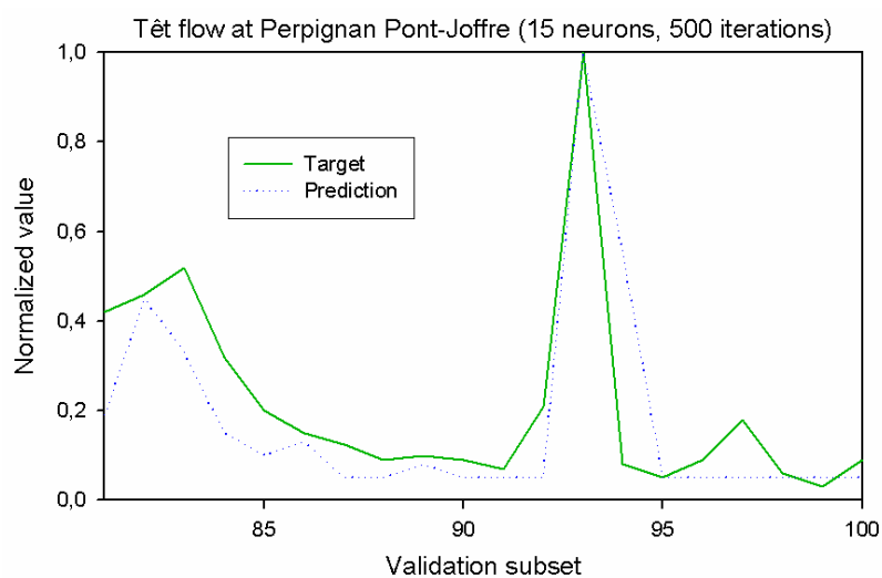
Fig. 6. Estimation results for the Têt flow at Perpignan Pont-Joffre (validation phase)
