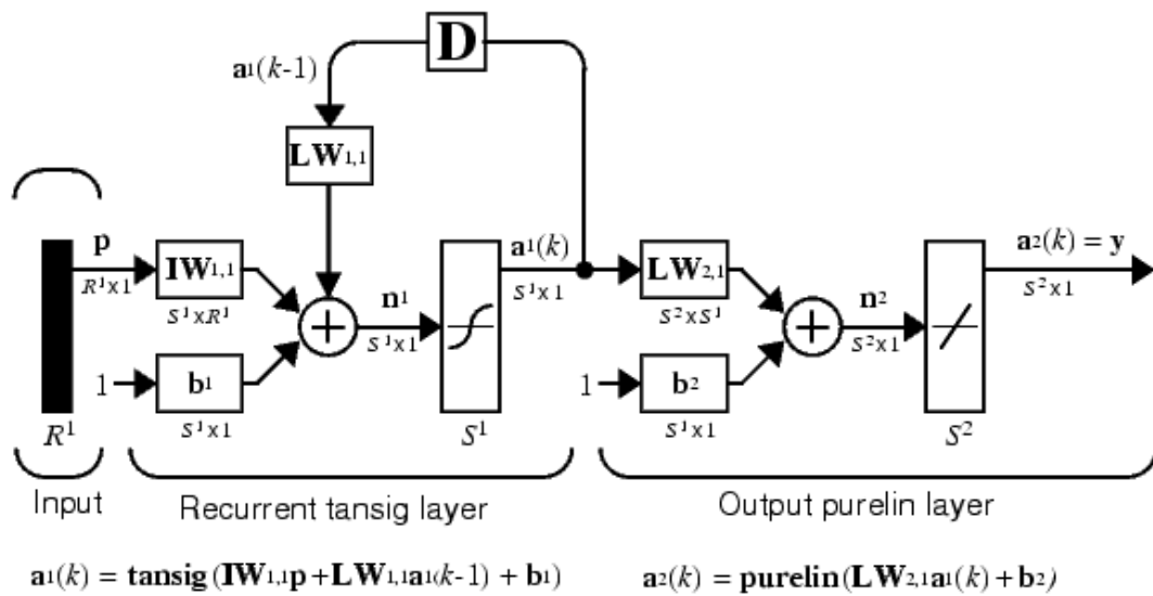
Fig. 2. A 2-layer Elman neural network
