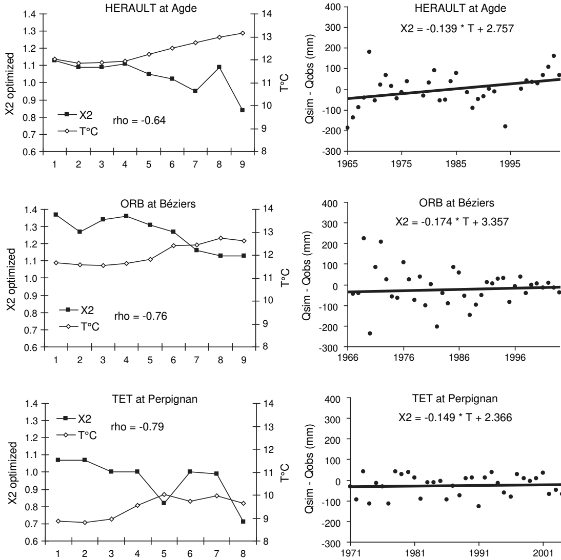
Fig. 11. Correction of the GR2M model drifts for the Hérault, Orb and Têt rivers. Left panels: Evolution of the optimized X_2 parameter value and mean annual temperature over the successive calibration periods. The rho values are the Spearman's correlation coefficients calculated between both time-series. Right panels: Time-series of differences (in mm) between the mean annual discharge simulated by the GR2M model with temperature-varying X_2 values and observations over the period 1965–2004.
