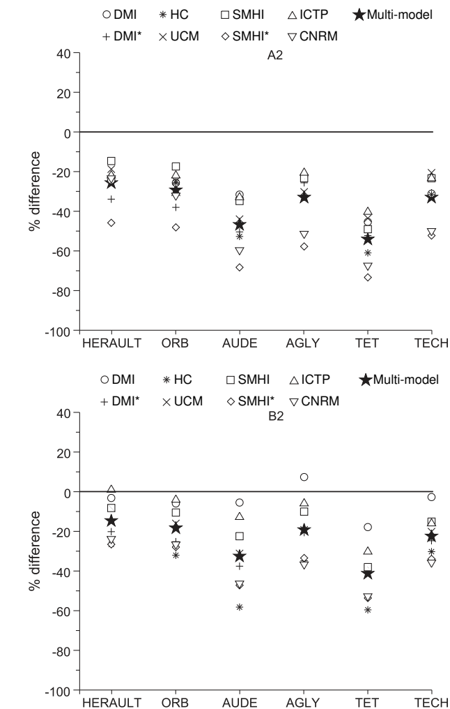
Fig. 6. Changes (in%) in the mean annual discharge simulated by the GR2M model calibrated over the 1965–1984 period (reference parameter set) between the periods 1961–1990 and 2071–2100. The RCMs marked with an asterisk were forced by the outputs of the GCM ECHAM4/OPYC3.
