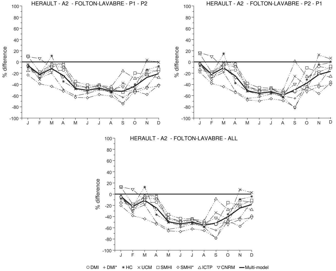
Fig. 10. Changes (in%) in the mean monthly discharge simulated by the GR2M model calibrated on different periods according to the full split-sample test of Klemeš (1986) between the periods 1961–1990 and 2071–2100 for the Hérault River for the A2 scenario. The RCMs marked with an asterisk were forced by the outputs of the GCM ECHAM4/OPYC3.
