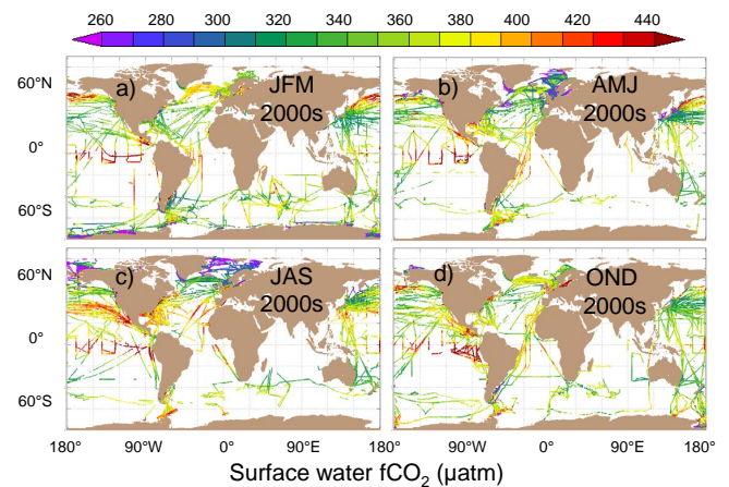
Figure 4. Seasonal distribution of surface water f\text{CO}_2 ( \mu\text{atm} ) for the months (a) January through March, (b) April through June, (c) July through September and (d) October through December in the years 2000 through 2009 in SOCAT version 3 for data sets with flags of A to E (after Bakker et al., 2014).
