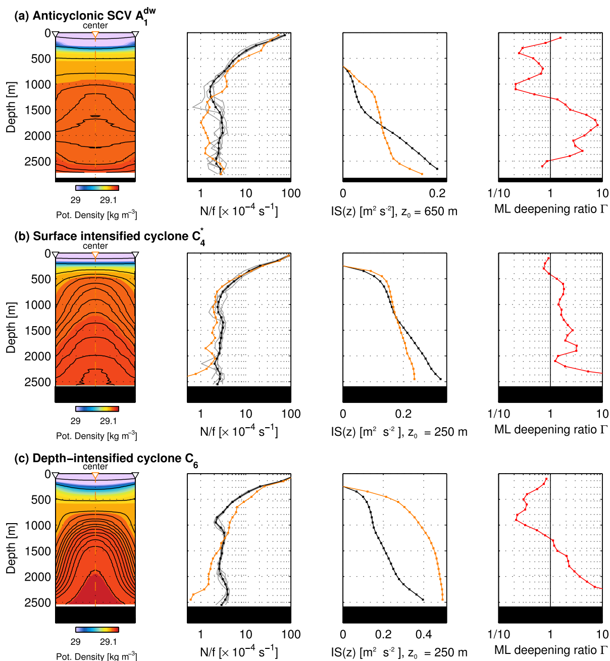
Figure 8. For (a) anticyclone A_1^{dw} , (b) surface-intensified cyclone C_4^* , and (c) depth-intensified cyclone C_6 sampled by R/Vs, we represent: (left) their density section from the far-field to the core; (middle left) the stratification normalized by the Coriolis parameter f for the far-field profiles in light gray, their mean in black and for the eddy core in orange; (middle right) the columnar buoyancy with depth integrated from a reference depth (650 m for (a) and 250 m for (b) and (c)) within the eddy in orange and in the far-field in black; (right) the mixed layer deepening ratio between the far-field and the eddy core. Note that the x axis is logarithmic for the middle left and the right plot.
