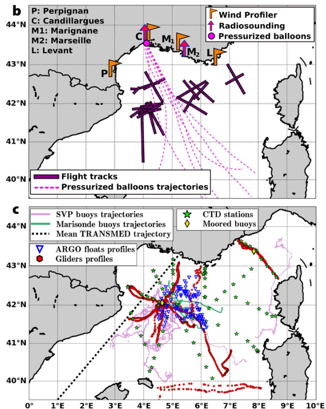
FIGURE 1. (a) Map of the northwestern Mediterranean. Red lines and arrows show the main oceanic characteristics. NC = Northern Current. BF = North Balearic Front. WCC = West Corsica Current. Green arrows show winds that typically contribute to dense water formation. (b) Fixed instruments and typical trajectories of the balloons and aircraft used to document the atmospheric boundary layer during HYdrological cycle in the Mediterranean Experiment (HyMeX) Special Observing Period 2 (SOP2). (c) Locations of the various HyMeX SOP2 platforms.
