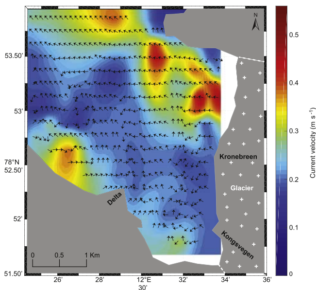
Fig. 5. Map of average current vectors at 3 m depth measured from 20 July to 3 August 2015. Arrows are normalized and indicate in which direction currents were going. A color scale is used to show current velocity ( \text{m s}^{-1} ). (For interpretation of the references to colour in this figure legend, the reader is referred to the Web version of this article.)
