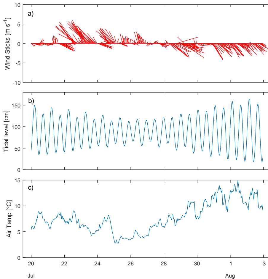
Fig. 3. From top to bottom: a) stick plot of wind speed and direction (by convention the stick plot indicates the direction from where the wind is blowing), b) tidal level and c) air temperature measured in Ny-Ålesund.
