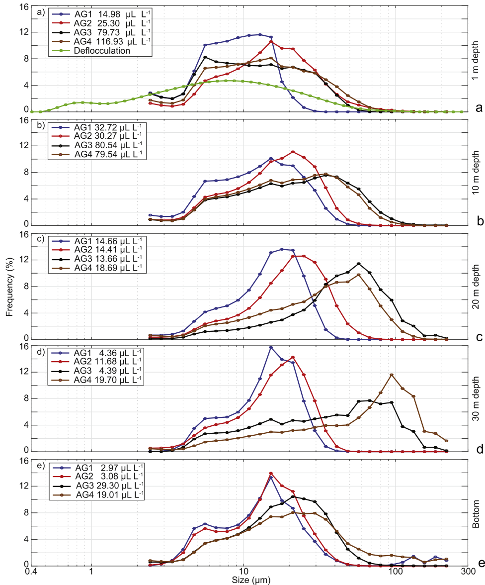
Fig. 7. Evolution of PSD from offshore towards the glacier front (station AG1 to AG4) a) at the surface (1 m), b) 10 m, c) 20 m, d) 30 m water depth and e) close to the bottom (1 meter above the bottom, mab) (e). See Fig. 1 for stations' location. In laboratory primary (deflocculated) PSD is shown in green on the top panel. (For interpretation of the references to colour in this figure legend, the reader is referred to the Web version of this article.)
