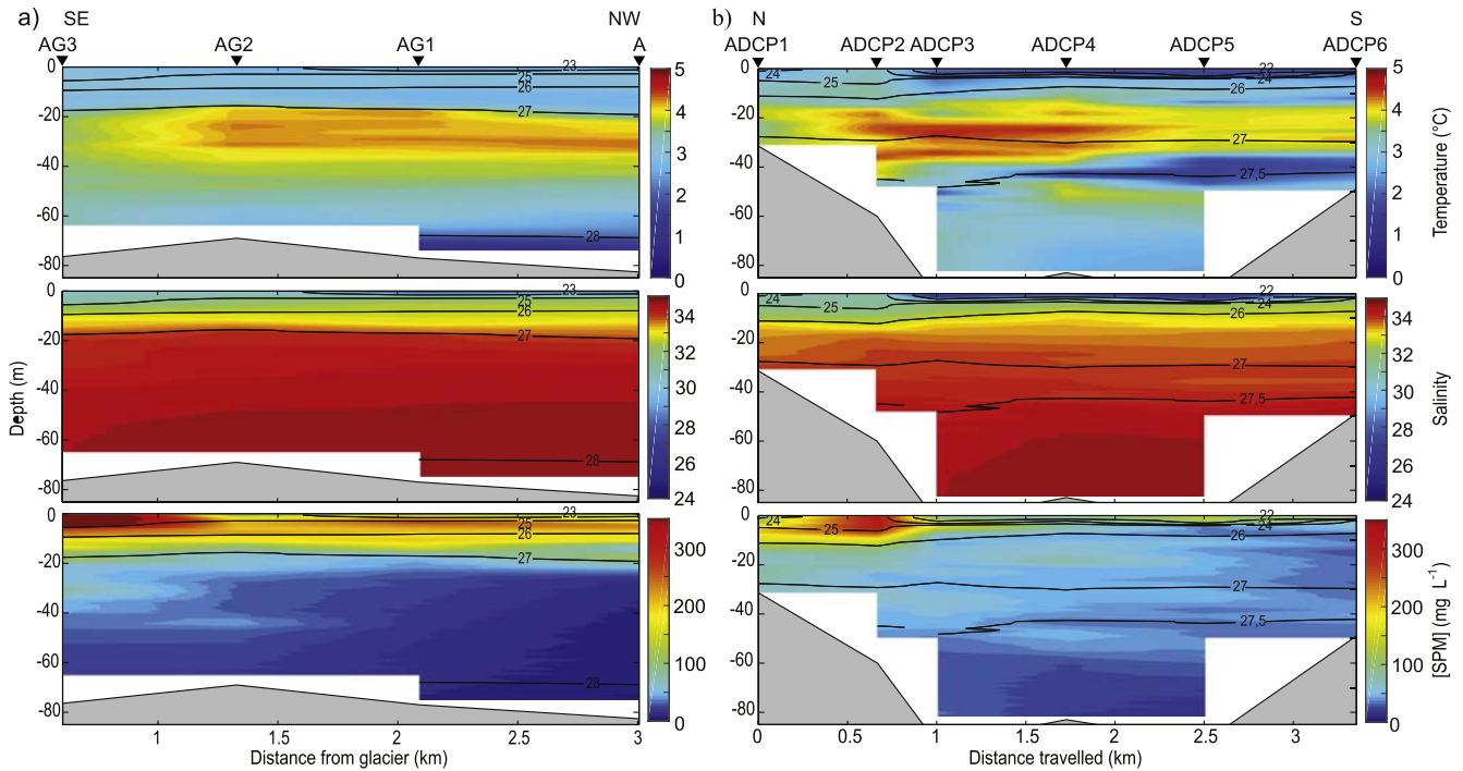
Fig. 4. a) SE-NW hydrological transect from CTD measurements on 31 July 2015. b) N-S hydrological transect parallel to the ice front measured on 3 August 2015. From top to bottom: temperature ( ^{\circ}\text{C} ), salinity and SPM concentrations ( \text{mg L}^{-1} ). Contour lines represent the seawater density ( \text{sigma-t} in \text{kg m}^{-3} ). The localisation of stations is indicated in the top plots by black triangles and are also indicated in Fig. 1c with the position of transects.
