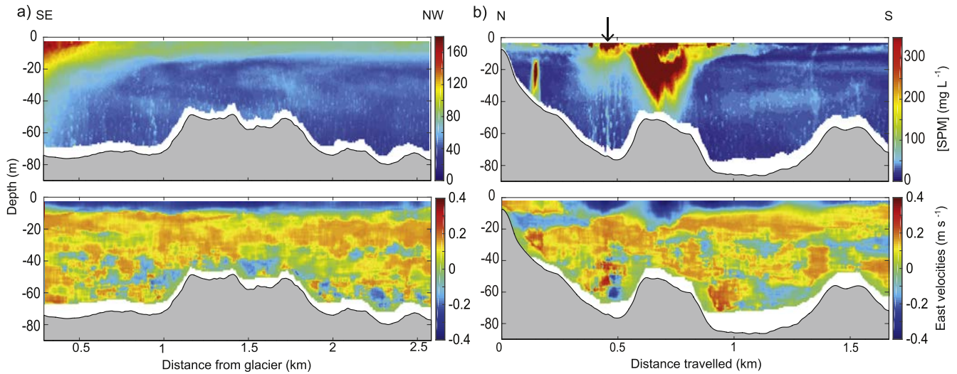
Fig. 6. a) ADCP SE-NW transect measured on 3 August 2015 and b) N-S transect measured on 31 July 2015 (see Fig. 1c for the localisation of transects). From top to bottom: acoustic-derived SPM concentration (in \text{mg L}^{-1} ) and horizontal current velocities ( \text{m s}^{-1} ). Positive values are eastwards currents and negative values are westwards currents. Note the different colorbar scales for SPM concentration for both transects. The position of the SE-NW transect (Fig. 6a) is indicated by the arrow above the N-S transect (Fig. 6b). (For interpretation of the references to colour in this figure legend, the reader is referred to the Web version of this article.)
