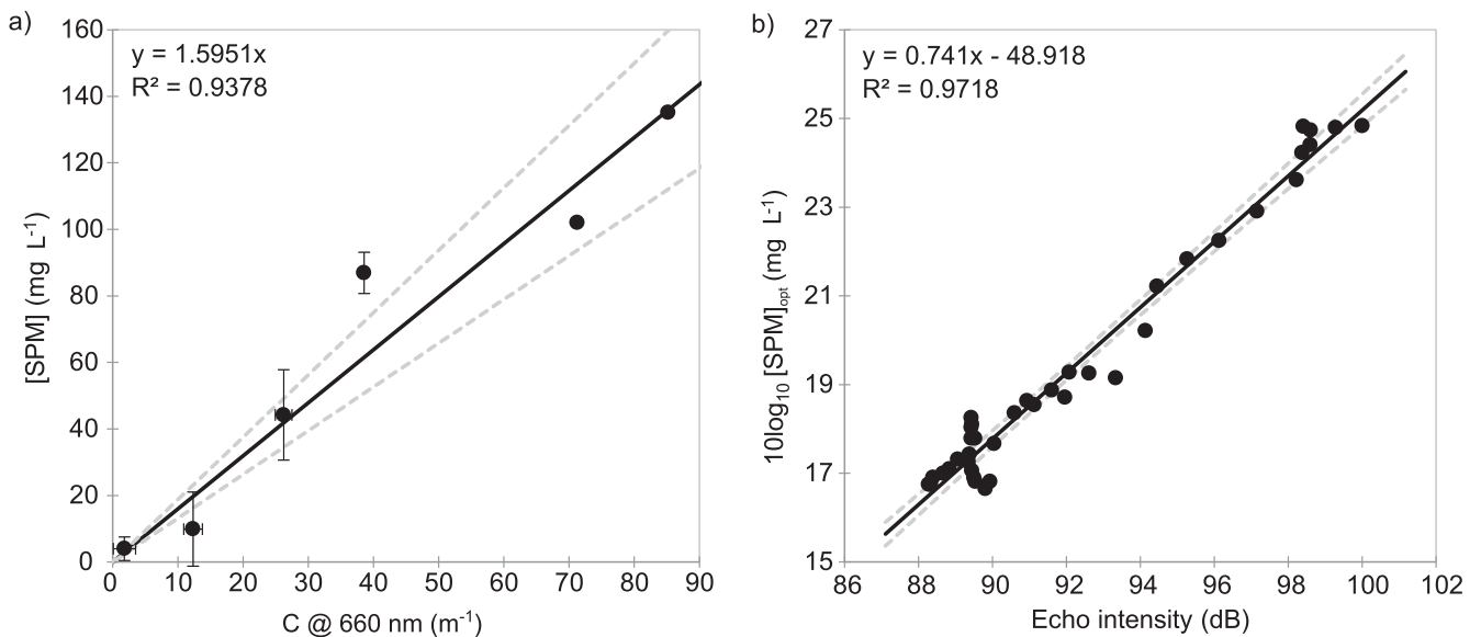
Fig. 2. a) Calibration curve of the attenuation coefficient c (660nm) of the LISST-100X vs in-situ SPM measurements. The standard deviation of each group is shown. Dashed lines represent the 95 % confidence interval of the regression. b) Calibration curve of the Echo Intensity (EI) of the ADCP vs optically derived SPM concentrations. Dashed lines represent the 95 % confidence interval of the regression.
