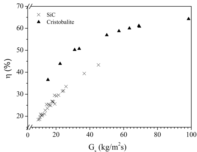
Figure 6. Calculated efficiency of the UBFB conveying.
