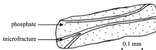
Figure 14. Phosphatic grain in longitudinal section.
