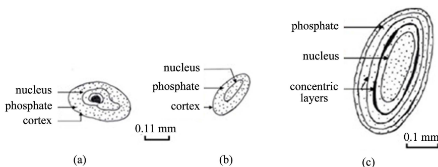
Figure 10. Epigenized oolites.
