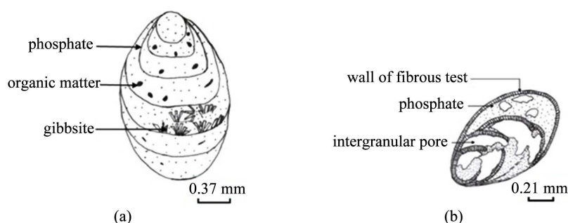
Figure 7. Daucina ermaniana obtusa : (a) Chambers filled with gibbsite; (b) Pores.
