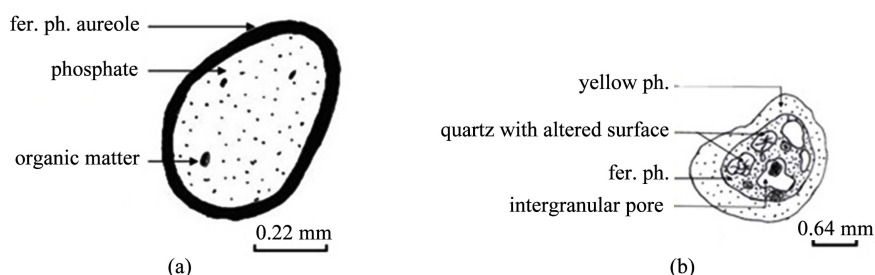
Figure 8. Phosphate grain (a) without endogangue; (b) with quartzose endogangue.
