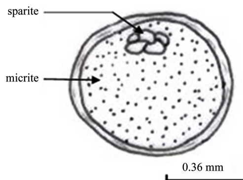
Figure 11. Coprolite in transverse section.
