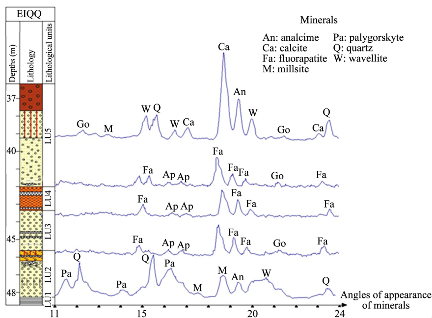
Figure 15. Lithology of the EIQQ borehole and the diffractograms of the analysed phosphate samples [10].
