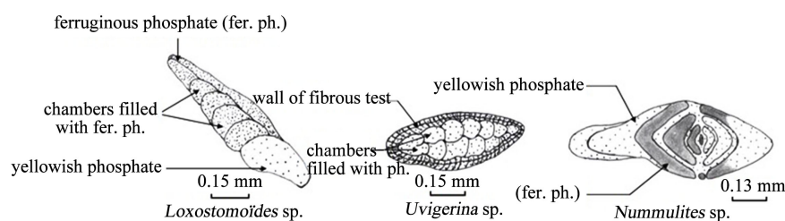
Figure 6. Foraminifera with epigenized test.
