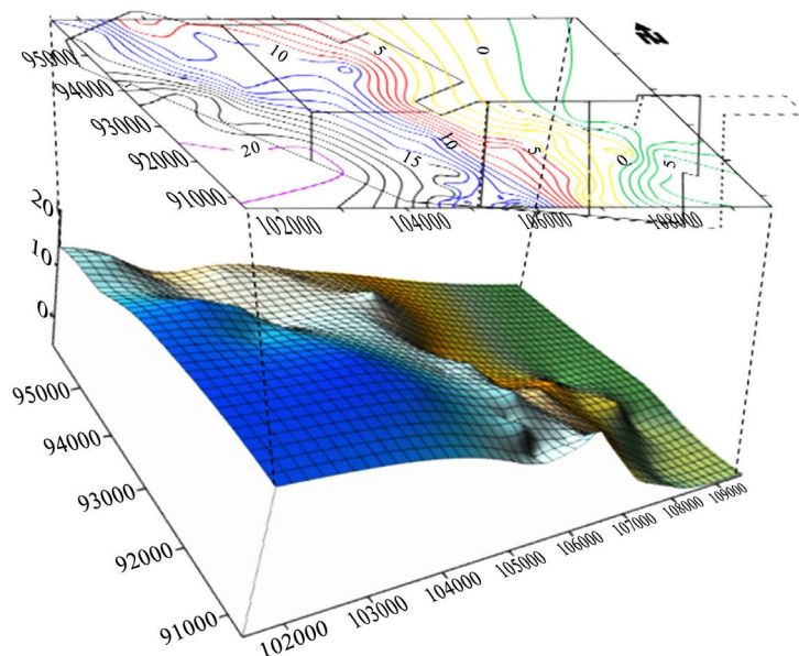
Figure 4. Three-dimensional view of the wall structure of Tobène.
