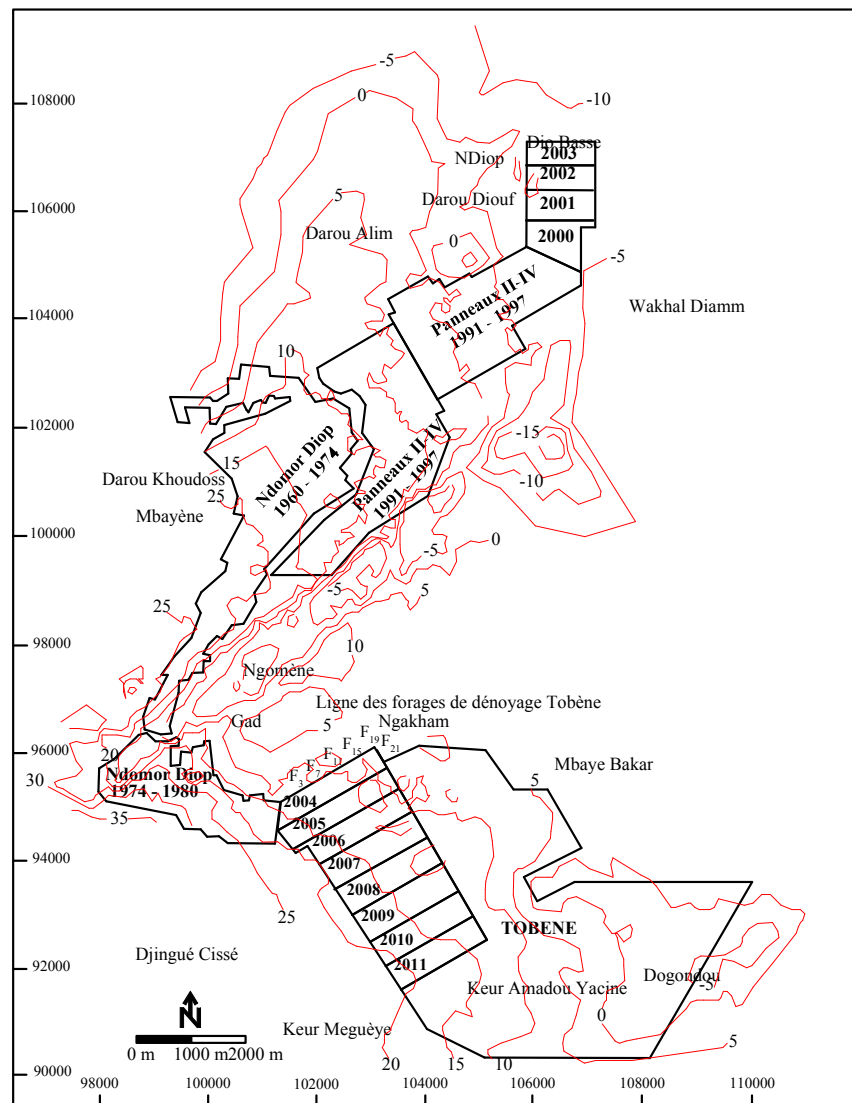
Figure 1. The main panels and isobath map of the wall of the Taïba deposit.
