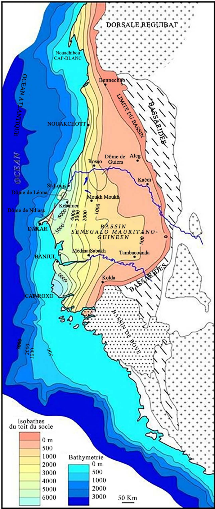
Figure 2. Regional context of the Senegal-Mauritania-Guinea sedimentary basin [1].
