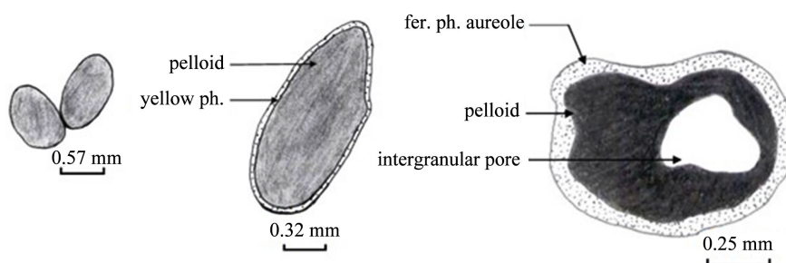
Figure 12. Peloids with variable forms and sizes.
