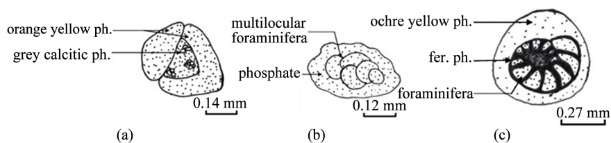
Figure 9. Phosphatic grain (a) with calcitic endogangue; (b) and (c) with bioclastic endogangue.
