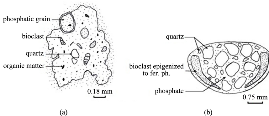
Figure 13. Phosphatic lithoclast.
