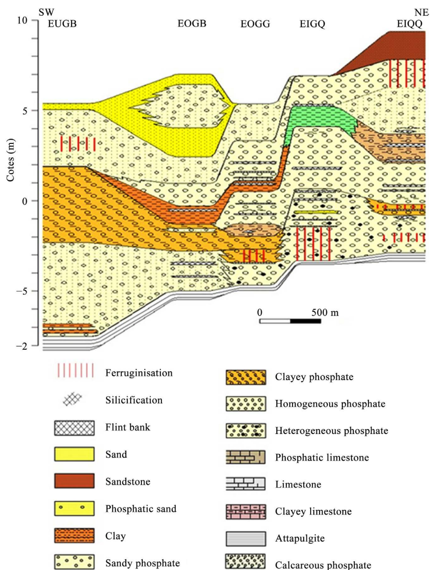
Figure 5. Lithological section of boreholes in the western sector [9].
