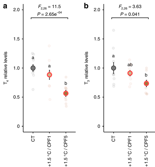
Fig. 4 Effects of increased temperature and chlorpyrifos co-exposure on TH levels. a, b Respective T_4 levels ( n = 29 ) and T_3 levels ( n = 29 ) in d2 A. triostegus exposed to increased temperature (CT = control, 28.5 °C; +1.5 °C = 30.0 °C) and CPF (CT = control, no CPF; CPF1 and CPF5 = CPF at 1 and 5 \mu\text{g L}^{-1} , respectively). Data are indicated as mean (opaque circles) \pm SE (error bars), and transparent circles indicate each data point. Letters indicate statistically different groups according to two-sided Tukey post hoc tests following LM ( F ). Source data are provided as a Source Data file.
