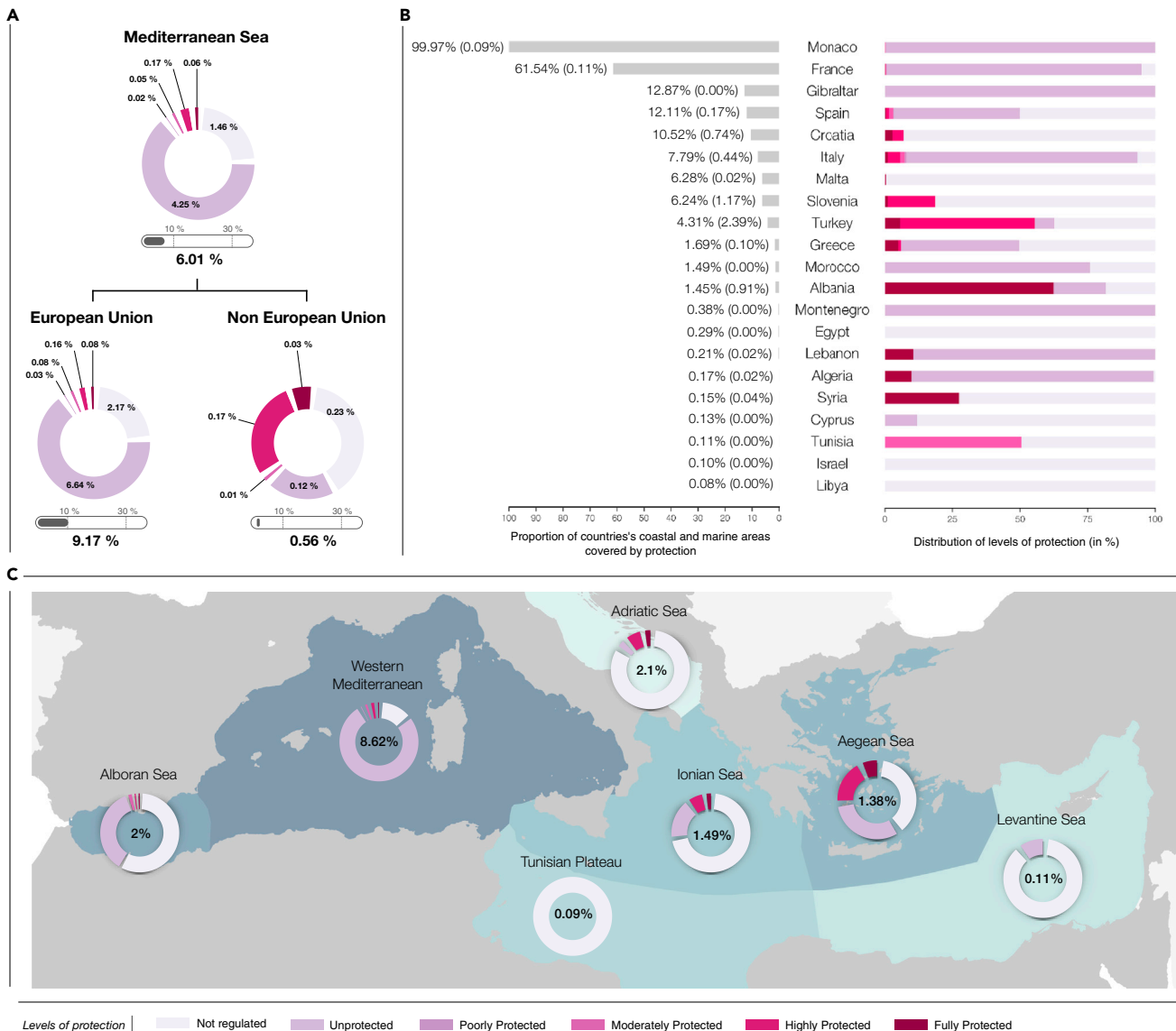
Figure 2. Distribution of the Different Levels of Protection in the Mediterranean Sea
