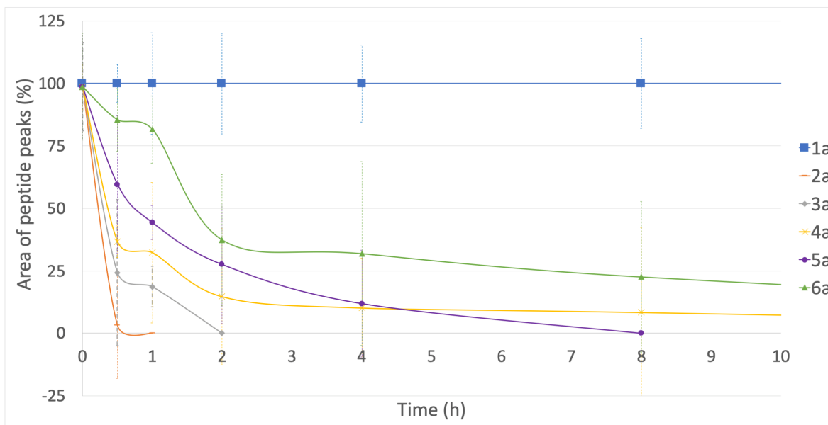
Figure 3. Cleavage rate of laxaphycin-B type peptides 2a-6a , compared to that of laxaphycin A 1a (averaged rate), as a function of the incubation time of the peptide with Dg-Ss-Lm . Error bars represent standard deviation.
