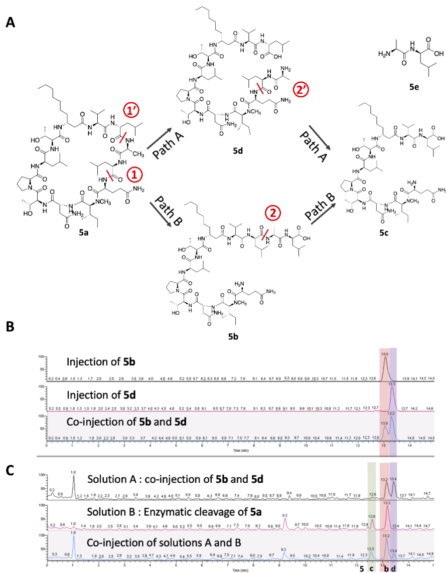
Figure 4. Study of the two possible enzymatic cleavage paths of compound 5a which leads to the formation of compounds 5c and 5e consecutively from the intermediates 5b or 5d . A. Potential intermediates produced by Path A or B. B. LC-MS chromatograms of postulated cleavage intermediates 5b (pink strip) and 5d (purple strip) and their co-injection. C. LC-MS chromatogram of 5a exposed to enzymatic degradation producing compound 5b as confirmed by co-injection with synthetic 5b and 5d compounds. Compound 5c resulting from the second cleavage is also observed (green strip).
