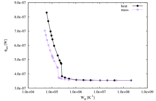
Figure 25: Total viscous dissipation as a function of W_\Phi .
