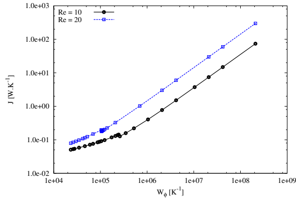
Figure 11: Objective functional J as a function of W_\Phi .
