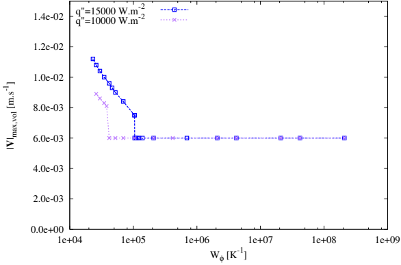
Figure 15: Maximum velocity magnitude in the channel as a function of W_\Phi for two values of the input heat flux.
