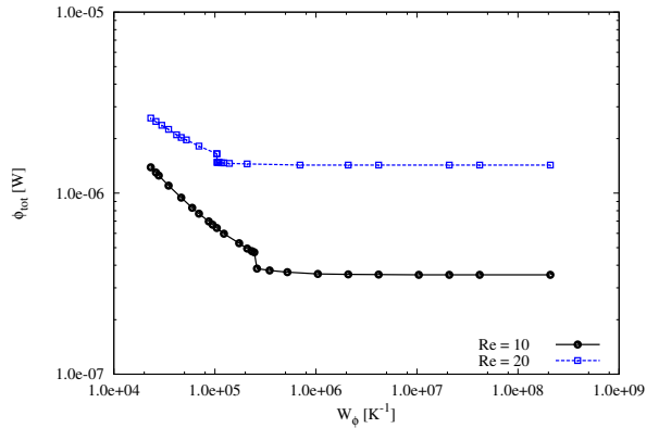
Figure 9: Total viscous dissipation as a function of W_\Phi .
