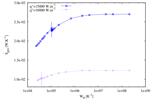
Figure 13: Total entropy generation rates as a function of W_\Phi for two values of the input heat flux. Re = 20 .
