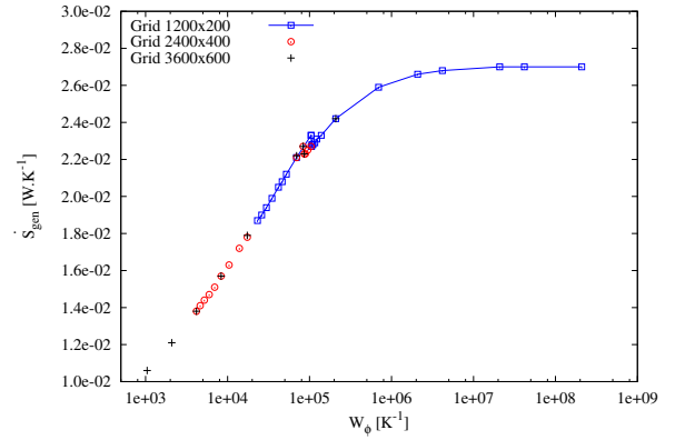
Figure 32: Total entropy generation rate as a function of W_{\Phi} , complemented by finer mesh simulations. Re = 20 .
