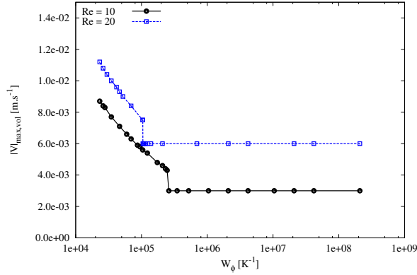
Figure 10: Maximum velocity magnitude in the channel as a function of W_\Phi .
