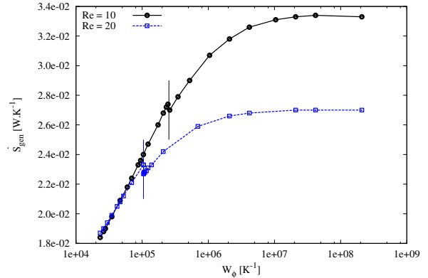
Figure 5: Entropy generation rate as a function of W_{\phi} .
