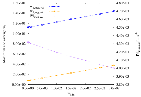
Figure 31: Maximum velocity magnitude in the channel as functions the inlet mass fraction of the minor species ( W_{\Phi} = 1.67 \times 10^5 K^{-1} and Re = 10 ).
