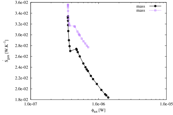
Figure 26: Total entropy generation rate as a function of the total dissipation.
