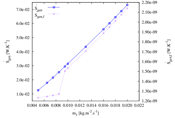
Figure 28: Total and viscous entropy generation rates as functions of the diffusion intensity from the bottom plate ( W_\Phi = 1.67 \times 10^5 K^{-1} and Re = 10 ).
