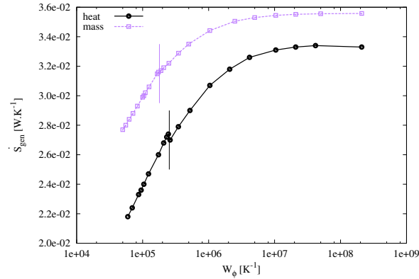
Figure 22: Total entropy generation rate as a function of W_\Phi .
