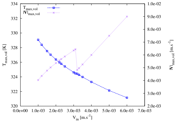
Figure 19: Maximum velocity magnitude and maximum scalar value in the channel as functions of V_{in} ( W_{\Phi} = 1.23 \times 10^5 K^{-1} ).
