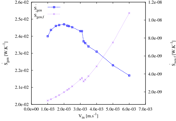
Figure 18: Total and viscous entropy generation rates as functions of V_{in} ( W_{\Phi} = 1.23 \times 10^5 K^{-1} ).
