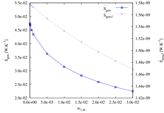
Figure 30: Total and viscous entropy generation rates in the channel as functions the inlet mass fraction of the minor species ( W_{\Phi} = 1.67 \times 10^5 K^{-1} and Re = 10 ).
