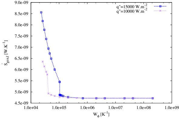
Figure 14: Total entropy generation rates by viscous friction as a function of W_\Phi for two values of the input heat flux.
