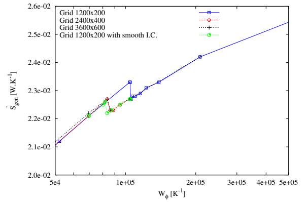
Figure 33: Total entropy generation rate as a function of W_{\Phi} - zoom on transition zone showing the influence of the grid resolution and the initial conditions (I.C.). Re = 20 .
