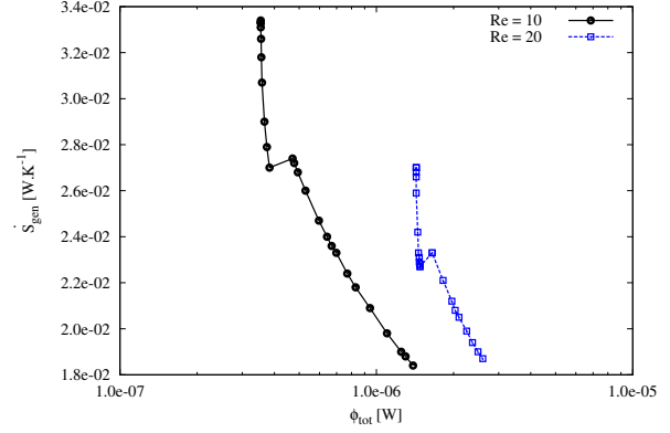
Figure 12: Total entropy generation rate as a function of the total dissipation.
