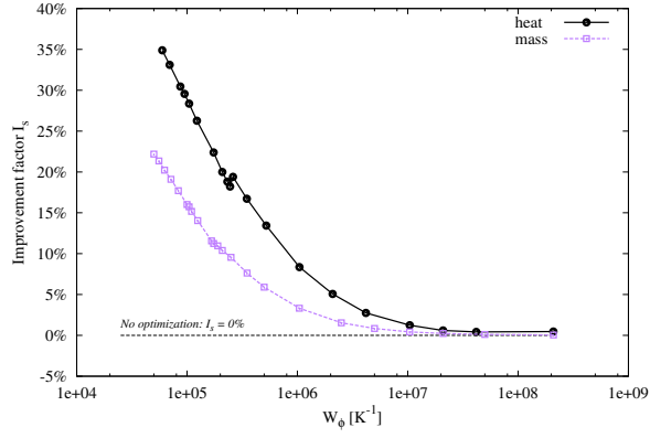
Figure 27: Improvement factor as a function of W_\Phi .
