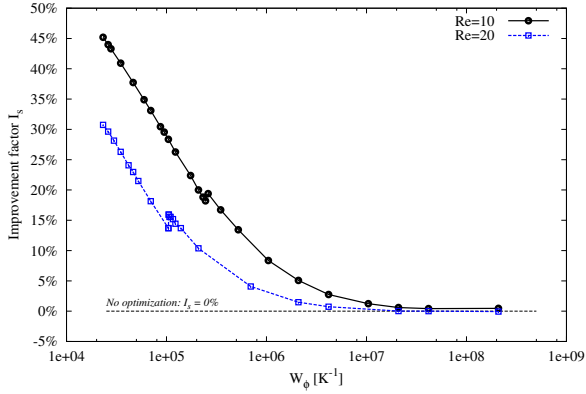
Figure 6: Improvement factor (Eq. 19) as a function of W_\Phi .
