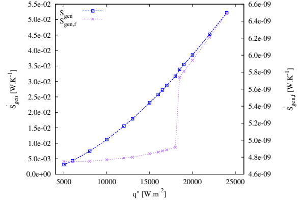
Figure 16: Total and viscous entropy generation rates as functions of the heat flux input from the bottom of the channel ( Re = 20 and W_\Phi = 1.23 \times 10^5 \text{ K}^{-1} ).
