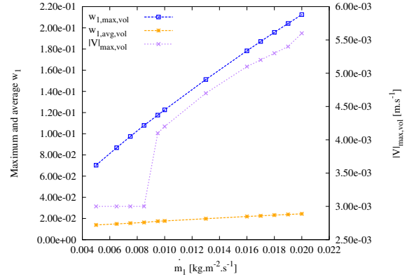
Figure 29: Maximum and average mass fraction of the minor species and maximum velocity as functions of the diffusion intensity from the bottom plate ( W_\Phi = 1.67 \times 10^5 K^{-1} and Re = 10 ).
