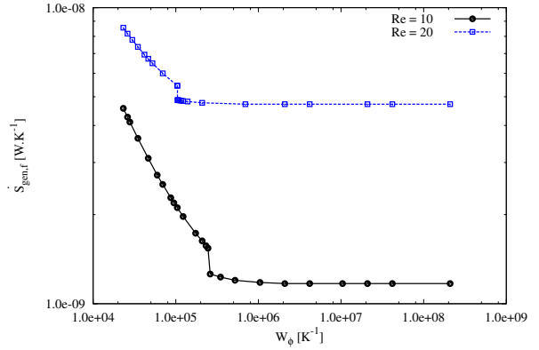
Figure 8: Entropy generation rate due to viscous friction as a function of W_\Phi .
