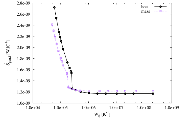
Figure 24: Entropy generation rate due to viscous friction as a function of W_\Phi .
