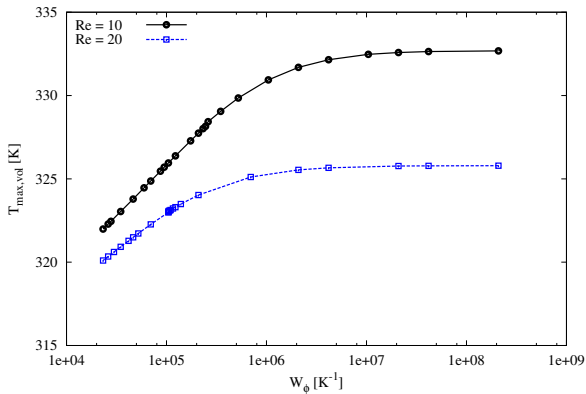
Figure 7: Maximum temperature in the channel as a function of W_\Phi .
