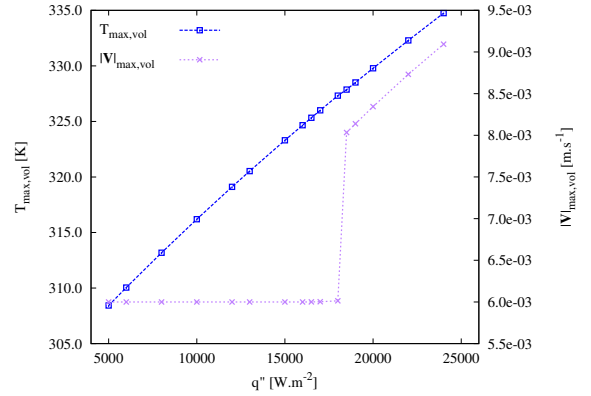
Figure 17: Maximum temperature and maximum velocity magnitude in the channel ( Re = 20 and W_\Phi = 1.23 \times 10^5 \text{ K}^{-1} ).
