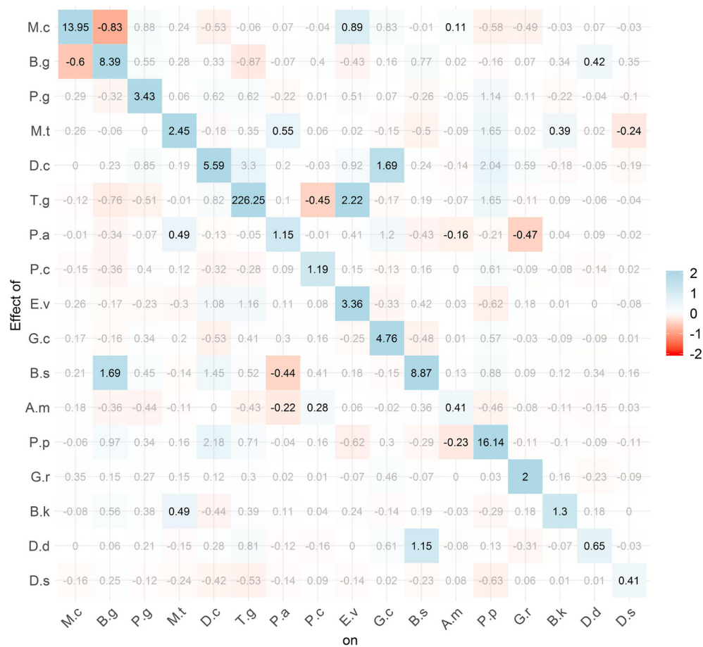
Figure 4. Effects of previous-year occupancy of other species. This effect was computed as [\Phi(\mu_i + \beta_j) - \Phi(\mu_i)]/\Phi(\mu_i) , with \mu_i the intercept for species i , \beta_j the estimated effect of species j on species i in probit scale and \Phi() the CDF of the standard normal distribution. Negative effects are depicted by red color, positive effects by blue color and color intensity reflects the strength of the effect. Cells are half-transparent and numbers are in grey when the 90% confidence interval was overlapping with 0 (on probit scale). Species acronyms: M.c : Marisa cornuarietis , B.g : Biomphalaria glabrata , P.g : Pomacea glauca , M.t : Melanoides tuberculata , D.c : Drepanotrema cimex , T.g : Tarebia granifera , P.a : Physa acuta , P.c : Pseudosuccinea columella , E.v : Eupera viridans , G.c : Galba cubensis , B.s : Biomphalaria schrammi , A.m : Aplexa marmorata , P.p : Pyrgophorus parvulus , G.r : Gundlachia radiata , B.k : Biomphalaria kubniana , D.d : Drepanotrema depressissimum , D.s : Drepanotrema surinamense .
