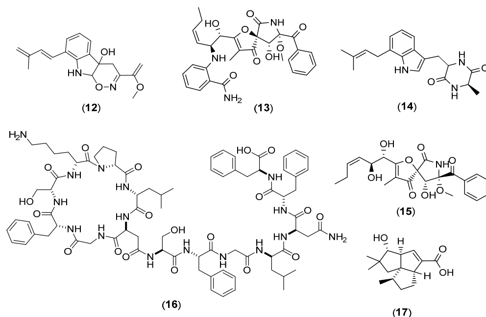
Figure 3. Chemical structures of luteotide D (12), pseurotin G (13), terezine D (14), 11-O-methylpseurotin A (15), chaxapeptin (16), and pentalenic acid (17).
