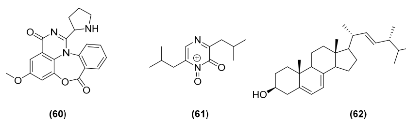
Figure 12. Chemical structures of aspergicin (60), neosaspergillilic acid (61), and ergosterol (62).
