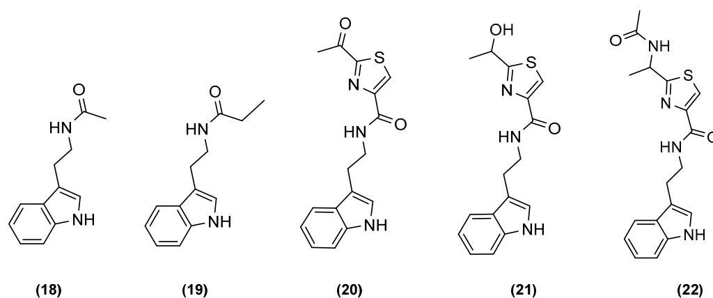
Figure 4. Chemical structures of the co-culture-induced compounds N -acetyltryptamine (18), N -propionyltryptamine (19), bacillamide A (20), bacillamide B (21), and bacillamide C (22).
