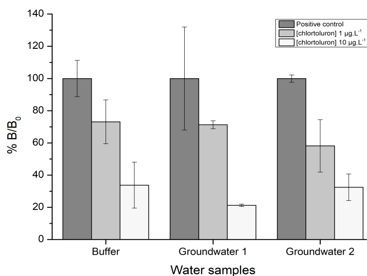
Figure 10. Electrochemical measurements of chlortoluron diluted at 1 and 10 \mu\text{g.L}^{-1} in two groundwaters and in the reference buffer PBS 1X pH 7.4.
