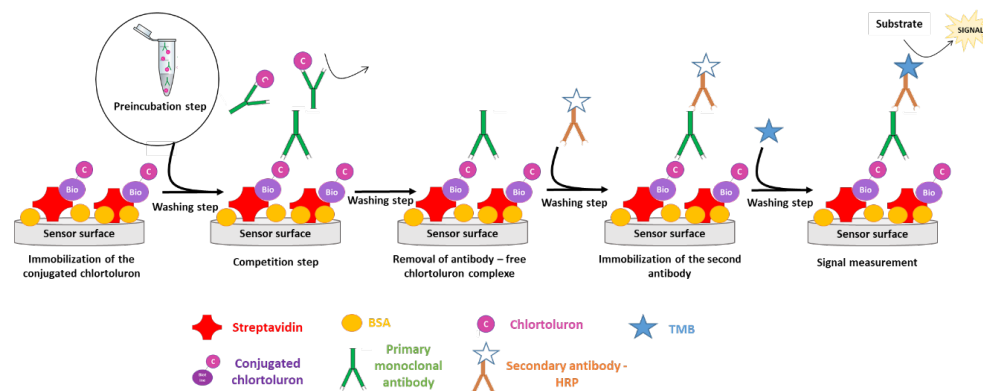
Figure 2. Description of the indirect detection based on the competition between immobilized conjugated chlortoluron and free chlortoluron for their binding to primary antibody.
