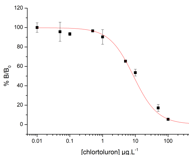
Figure 5. Calibration curve ( R^2 = 0.999 ) showing %B/B 0 versus chlortoluron concentrations, obtained with chlortoluron concentrations of 0; 0.05; 0.1; 0.5; 1; 5; 10; 50; 100 and 500 \mu\text{g.L}^{-1} .
