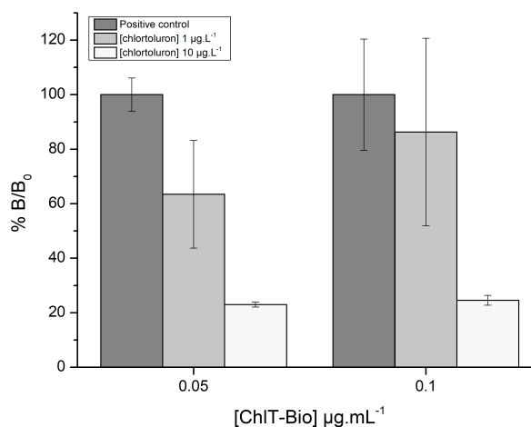
Figure 8. Relative response showing \%B/B_0 obtained for chlortoluron detection ( 1 \mu\text{g.L}^{-1} and 10 \mu\text{g.L}^{-1} ) using electrodes coated with biotinylated chlortoluron (ChIT-Bio) at 0.05 or 0.1 \mu\text{g.mL}^{-1} . Streptavidin and primary antibody concentrations were fixed at 5 \mu\text{g.mL}^{-1} and 0.6 \mu\text{g.mL}^{-1} , respectively.
