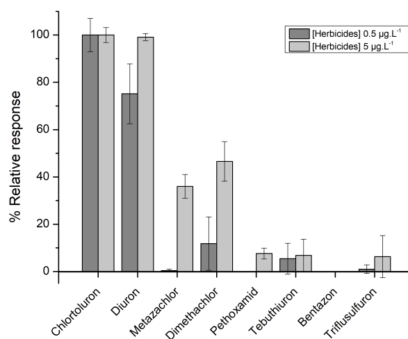
Figure 6. Relative response obtained in the presence of several herbicides compared to chlortoluron at concentrations of 0.5 and 5 \mu\text{g.L}^{-1} .
