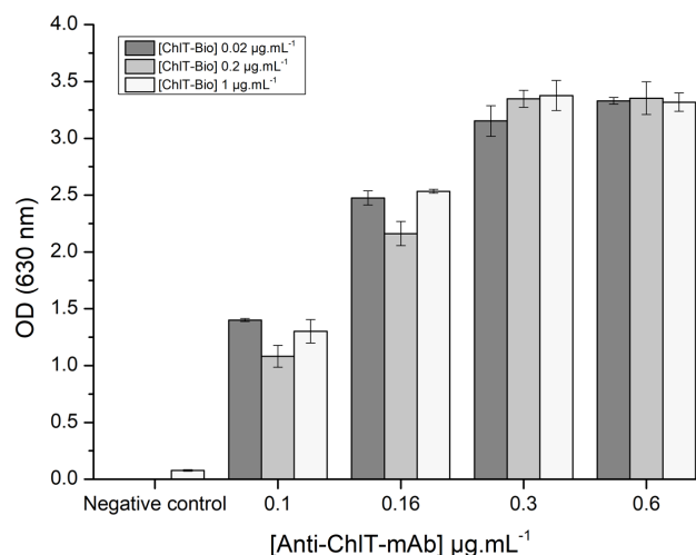
Figure 3. Absorbances measured using microplates coated with biotinylated chlortoluron (ChIT-Bio) at different concentrations (0.02, 0.2, 1 \mu\text{g.mL}^{-1} ) and using increasing concentrations of monoclonal antibody (Anti-ChIT-mAb) (0.1, 0.16, 0.3, 0.6 \mu\text{g.mL}^{-1} )
