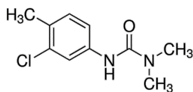
Figure 1. Molecular structure of chlortoluron herbicide.
