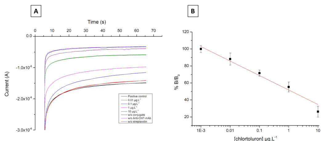
Figure 9. A. Chronoamperograms recorded after incubation with chlortoluron concentrations at 0 (positive control), 0.01, 0.1, 1 and 10 \mu\text{g.L}^{-1} . Applied potential -0.2 V vs Ag/AgCl. Negative controls measured without streptavidin, conjugated chlortoluron and primary antibody, respectively. B. Calibration curve presenting %B/B 0 versus chlortoluron concentrations ( R^2 = 0.96 ).
