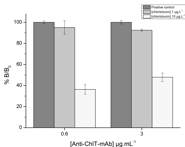
Figure 7. Relative response showing %B/B 0 obtained in presence of antibody (Anti-ChlT-mAb) at 0.6 and 3 \mu\text{g.mL}^{-1} , in presence of chlortoluron at 1 or 10 \mu\text{g.L}^{-1} . Streptavidin and biotinylated chlortoluron concentrations were set at 5 \mu\text{g.mL}^{-1} .
