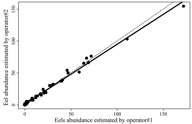
Fig. 1. Orthogonal regression (solid black line) of the estimated eel counts from 15 mn videos ( N=58 ) made by operators#1 and #2. The dashed line represents the line with a null intercept and a slope of one.
