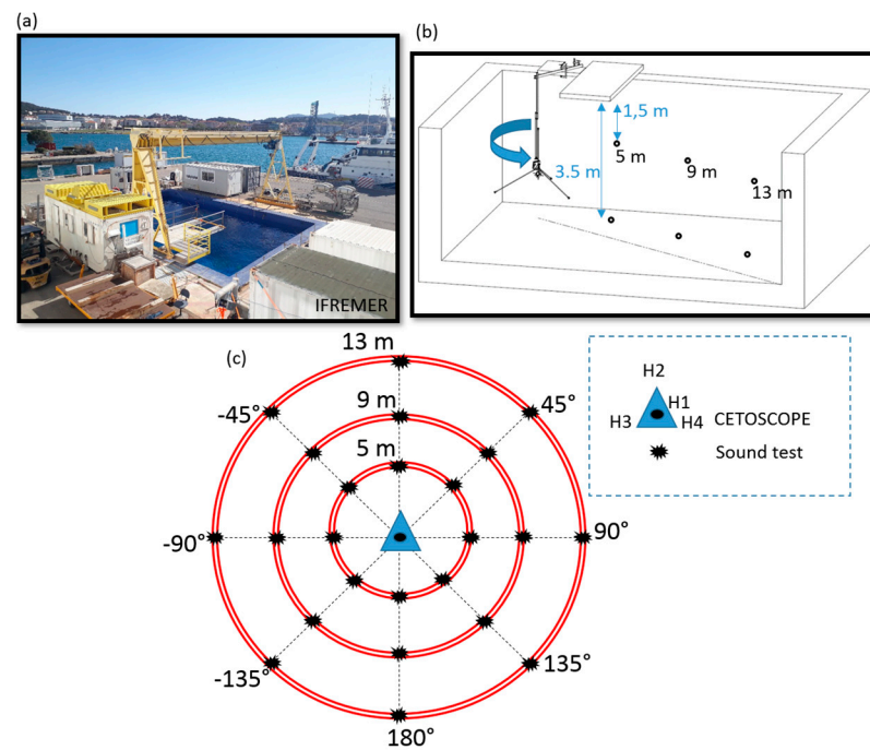
Figure 4. (a) view of the IFREMER (La Seyne/Mer) experimental pool, (b) side representation of the pool experiment protocol, (c) top view of the successive speaker positions.
