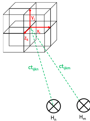
Figure 3. Geometric definition of the propagation distance between a given cubic mesh and a given pair of hydrophones n m.
