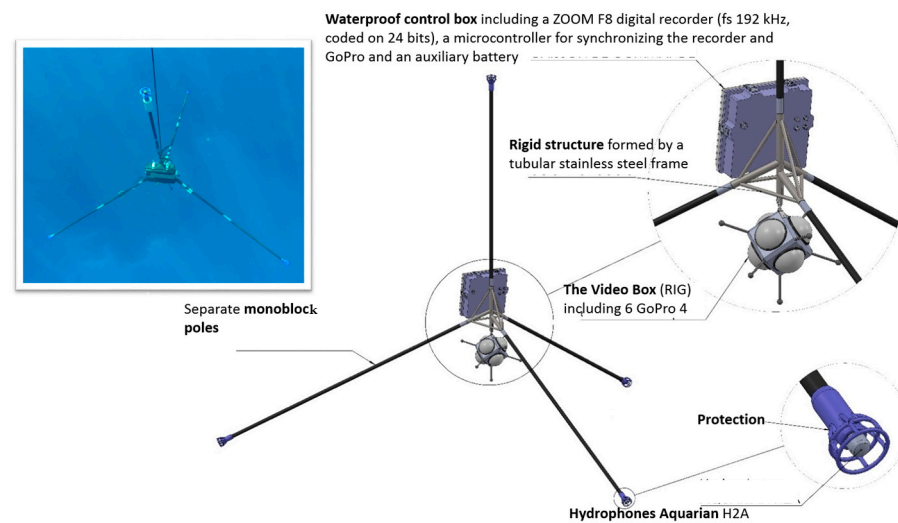
Figure 1. Description of the materials used for the CETOSCOPE©: a frame built with tubular stainless steel to make the overall structure rigid; 4 hydrophones, 1 placed at the extremity of each pole; the 360° video camera placed in the center; and the box including the digital recorder and the power battery.
