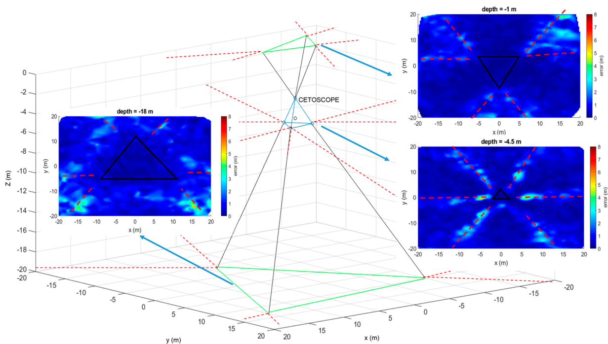
Figure 9. Relationship between geometrical projections of the array and changes in the shape of the shadow areas.
