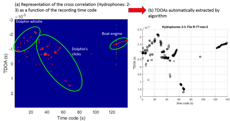
Figure 2. (a) Sliding cross-correlation of the signal over 130 s for a given pair of hydrophones. Time frame of 12.5 ms. Red dots represent the maximum of the cross-correlation by time frame and green ovals indicate the type of event confirmed by a human expert. (b) Automatically extracted TDOAs for the same sequence.
