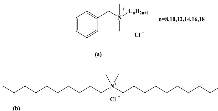
Figure 1. Chemical structures of BAC (a) and DDAC (b) biocides.
