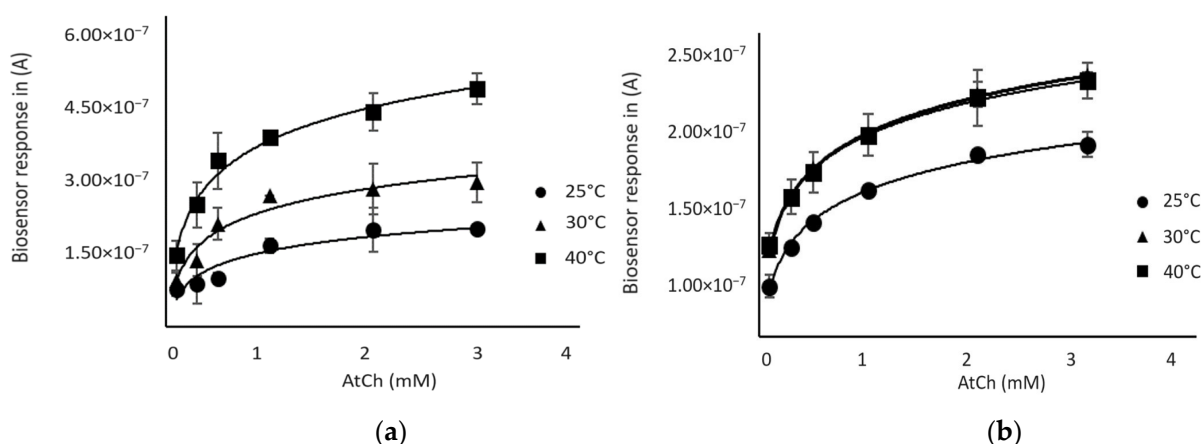
Figure 3. Response of the biosensor as a function of substrate (AtCh) concentration at different temperatures: (a) BChE-based biosensor (b) AChE-based biosensor.
