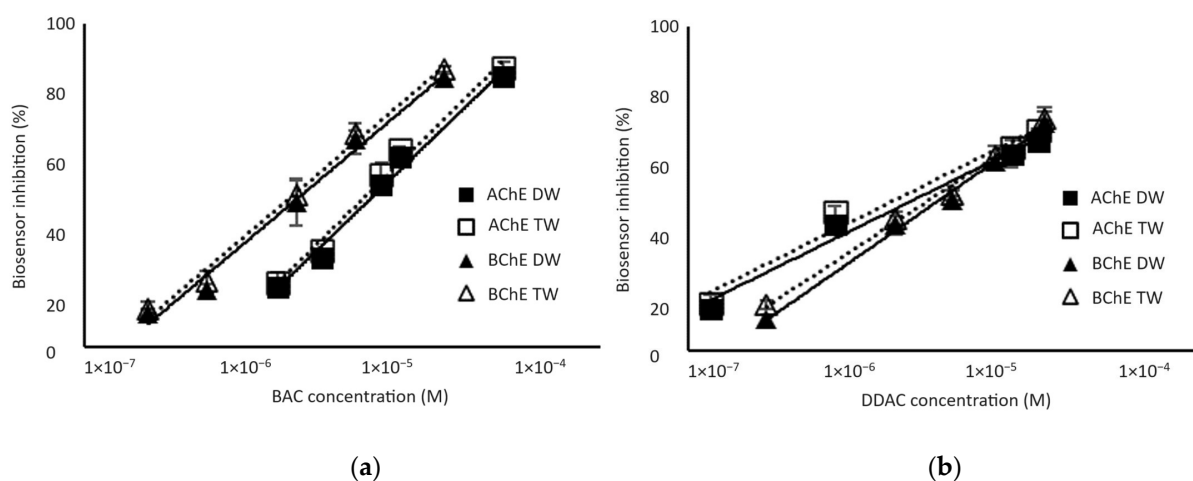
Figure 4. Inhibition effect of BAC (a) and DDAC (b) biocides on AChE- and BChE-based biosensors. Biocides were either prepared in distilled water (DW) or tap water (TW). Equations of the obtained curves are the following: (a) AChE-DW: y = 19.273\ln(x) + 271.23 ( R^2 = 0.9864 ); AChE-TW: y = 19.625\ln(x) + 277.62 ( R^2 = 0.9863 ); BChE-DW: y = 16.775\ln(x) + 261.12 ( R^2 = 0.9883 ); BChE-TW: y = 16.952\ln(x) + 265.6 ( R^2 = 0.9913 ). (b) AChE-DW: y = 9.7538\ln(x) + 176.67 , R^2 = 0.9839 ; AChE-TW: y = 9.8656\ln(x) + 181.03 ( R^2 = 0.9736 ); BChE-DW: y = 13.757\ln(x) + 221.11 ( R^2 = 0.9935 ); BChE-TW: y = 12.983\ln(x) + 213.91 ( R^2 = 0.9920 ).
