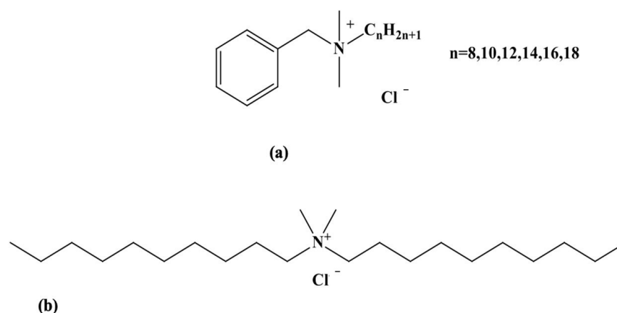
Figure 1. Chemical structures of BAC (a) and DDAC (b) biocides.
