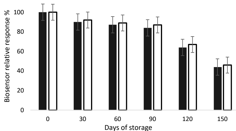
Figure 5. Relative response of AChE (dark bars) and BChE (white bars) biosensors during storage at 4 °C. The biosensor response was tested in presence of acetylthiocholine at 1 mM, as described in inhibition experiments.
